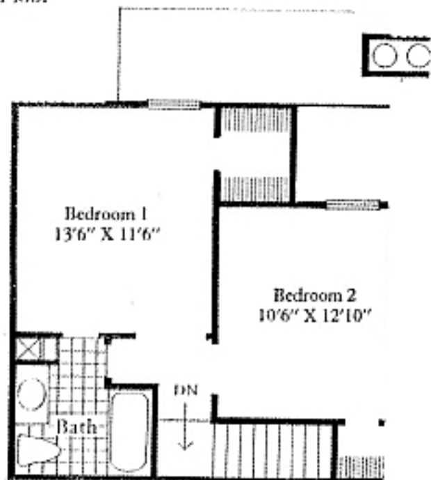
Third Floor
